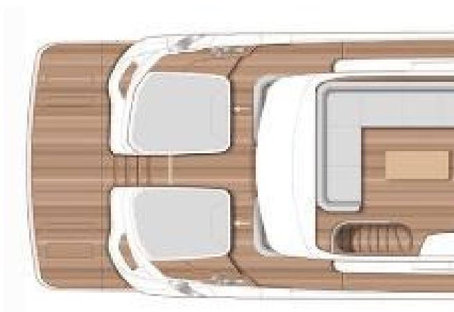
Princess S78 Sportsdeck Layout Plan
