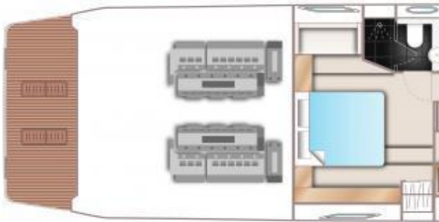
Manufacturer Provided Image: Princess V52 Lower Deck Layout Plan
